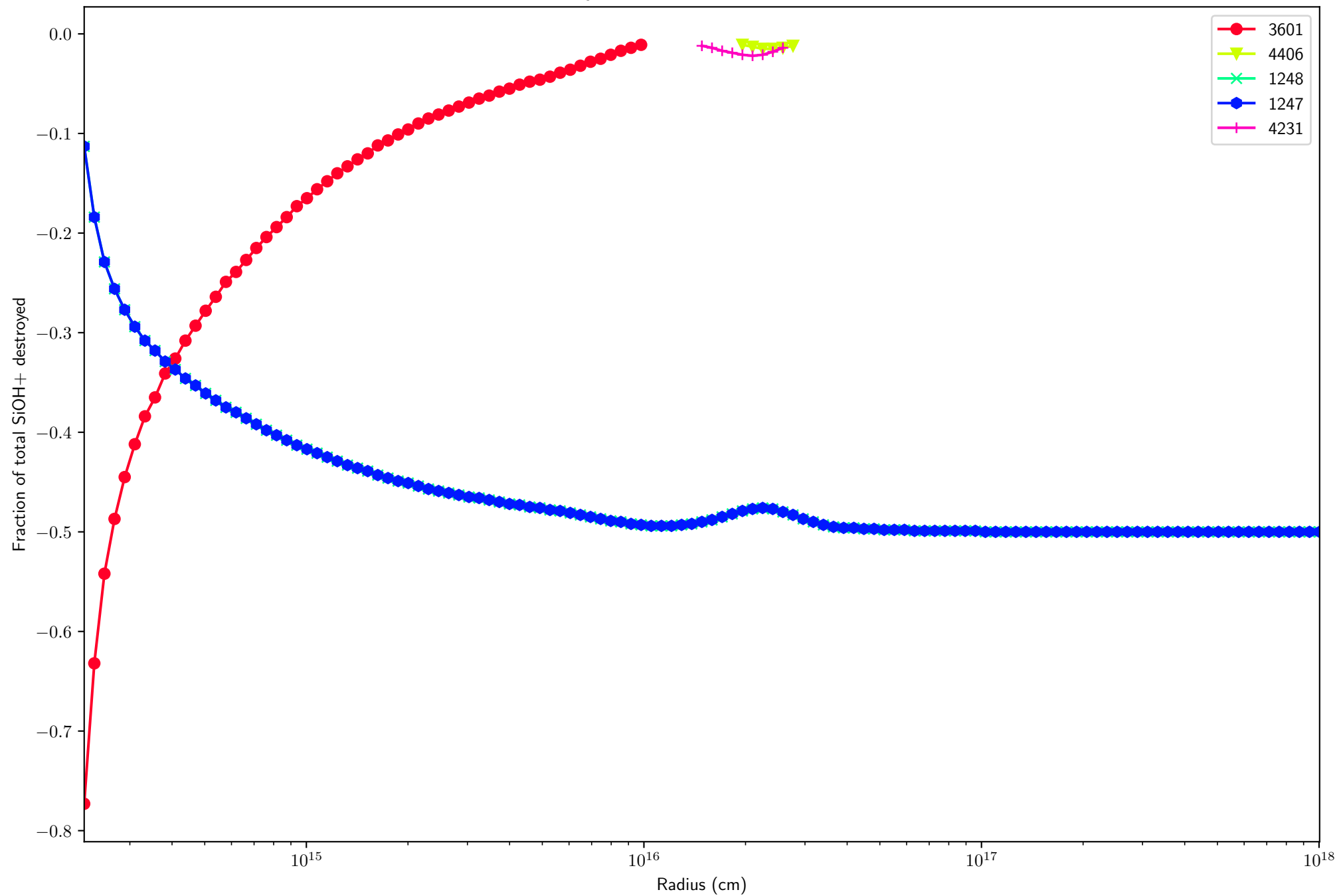
destruction-major-0-SiOH+-model-2025-10-27h15-32-23
